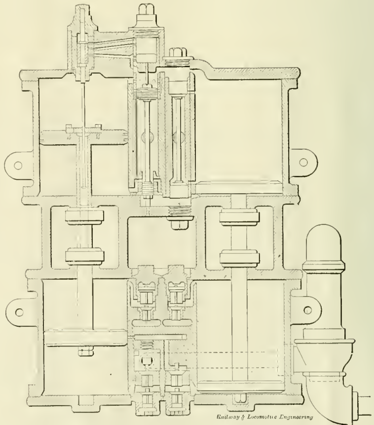
SECTIONAL VIEW OF MARSH'S COMPOUND AIR PUMP.
